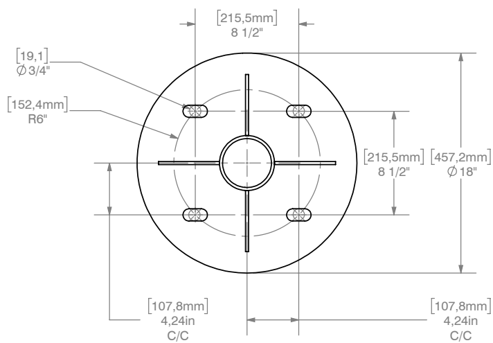
ANCHOR PLATE
