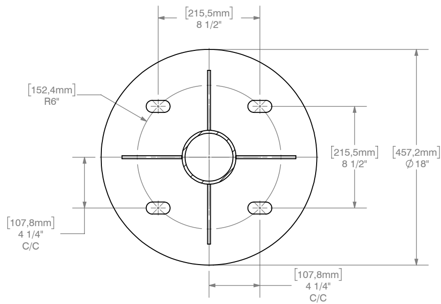
TYPICAL DETAIL ANCHOR PLATE
